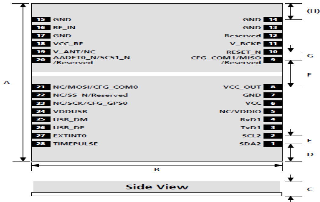
Figure 2: GT-2217-UB Pin Packag
